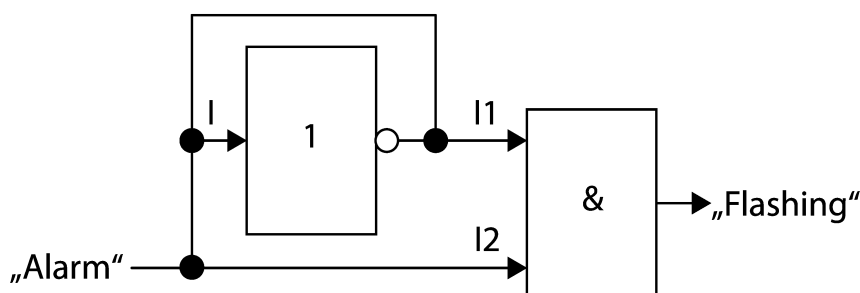
Figure 20: "Flashing" diagram
