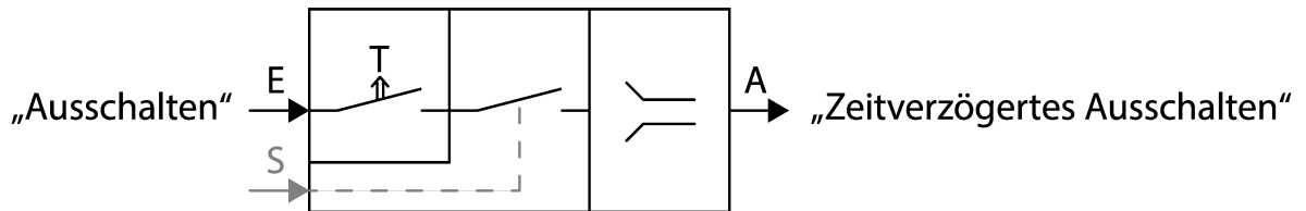
Figure 18: "Delayed switch-off" diagram
