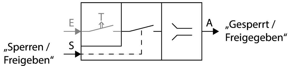
Figure 21: "Disabling function" diagram
