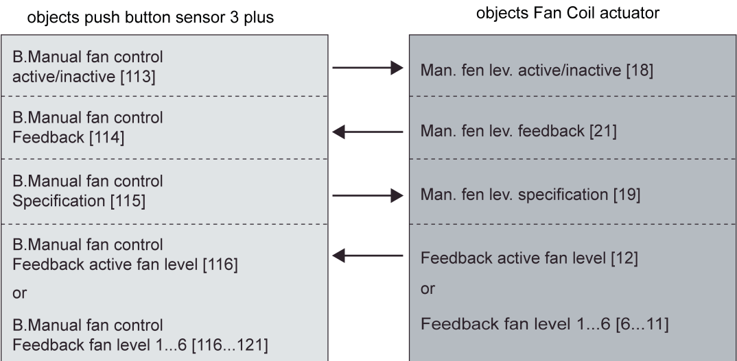
Figure 68: Communication objects of the manual fan control (1-to-1 linking with objects of the fan coil actuator with the same functions)
