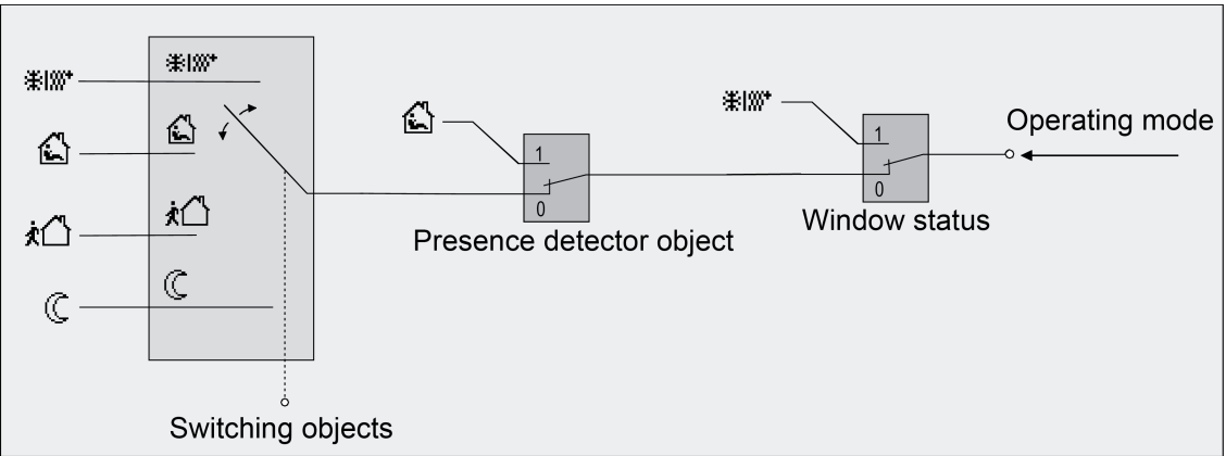
Figure 43: Operating mode change-over through 4 x 1-bit objects with presence detector
