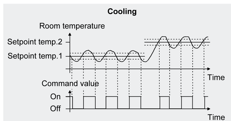
Figure 37: 2-point feedback control for the single "Cooling" operating mode
