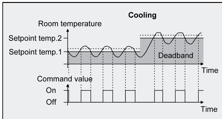
Figure 39: 2-point feedback control for mixed "Heating and cooling" mode with active cooling operation.
