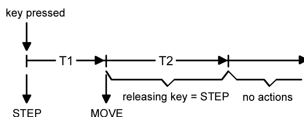
Figure 25: Operation concept "short – long – short"
