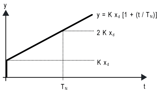
Figure 40: Function of the command value of a PI control
