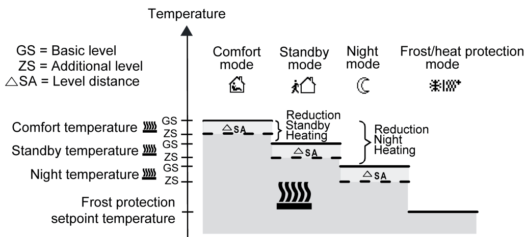
Figure 47: Setpoint temperatures in the operating mode "Basic and additional heating"
