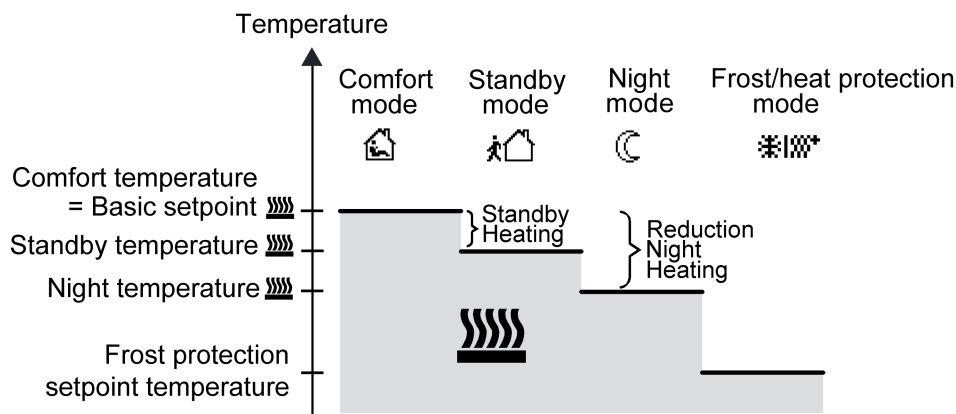
Figure 46: Setpoint temperatures in the operating mode "Heating"
