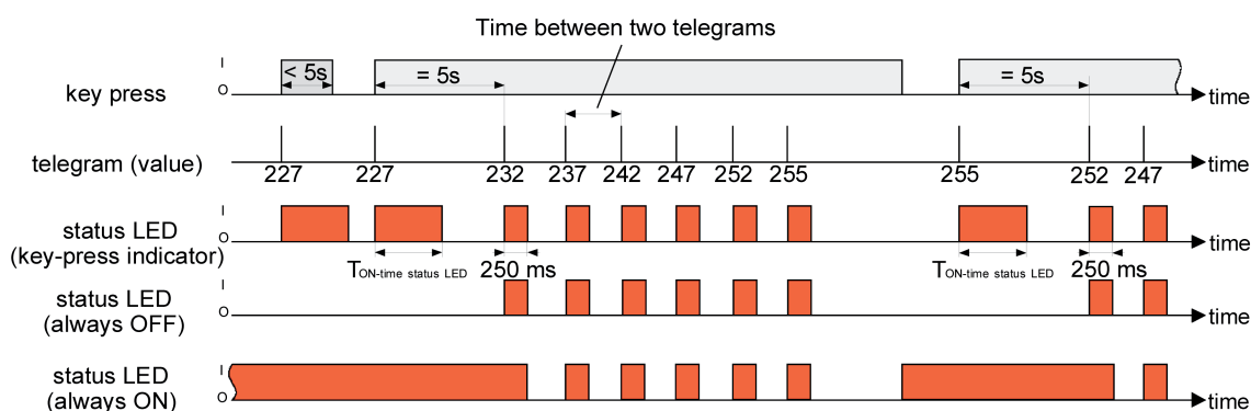
Figure 29: Example of value adjustment without value range overflow
