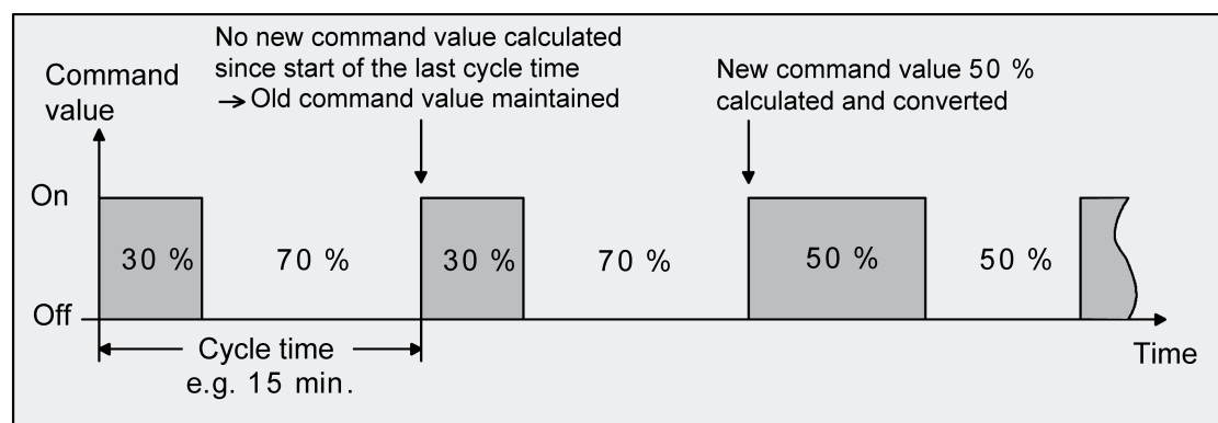
Figure 35: Switching PI control
