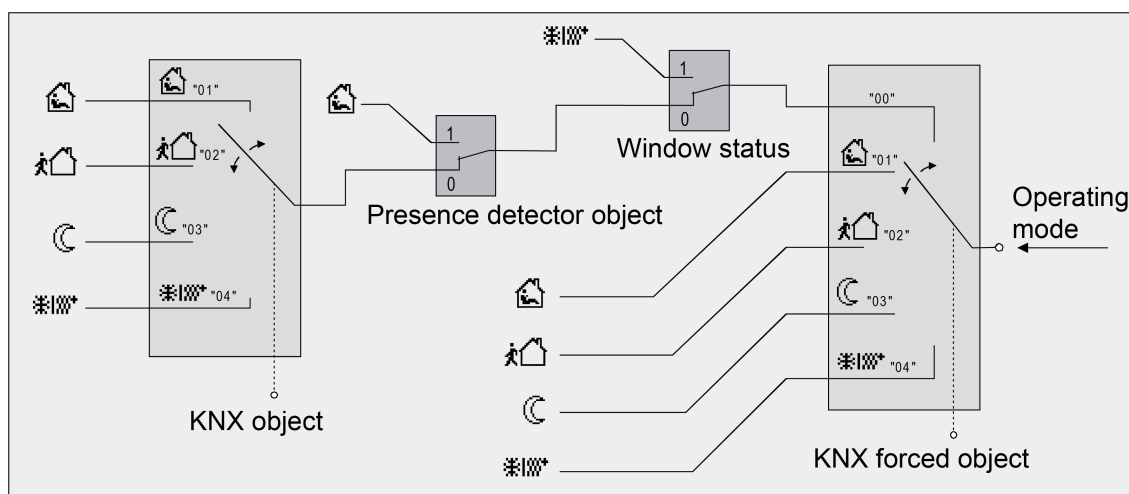
Figure 45: Operating mode change-over through KÖNEX object with presence detector
