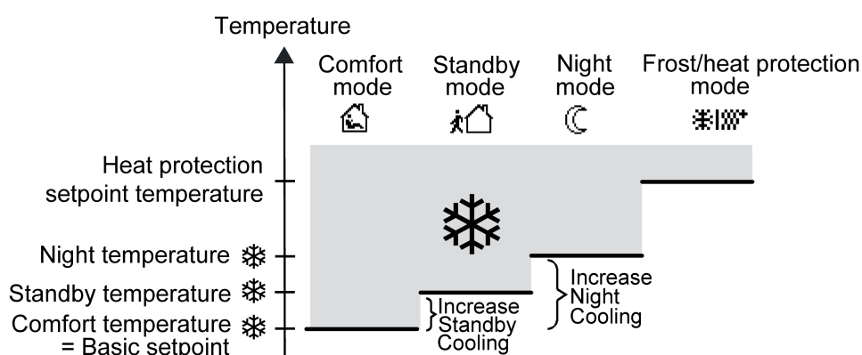
Figure 48: Setpoint temperatures in the operating mode "Cooling"
