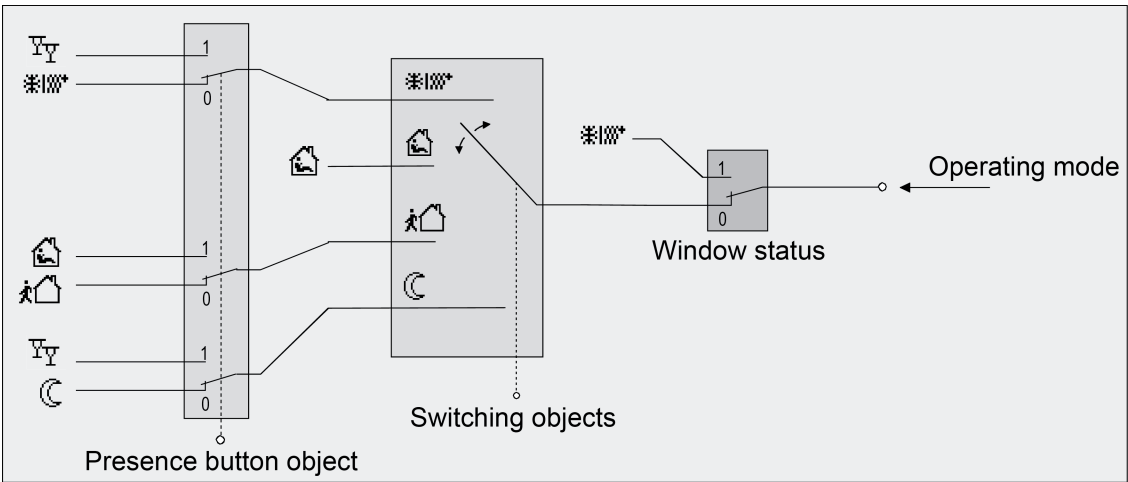
Figure 42: Operating mode change-over through 4 x 1-bit objects with presence button
