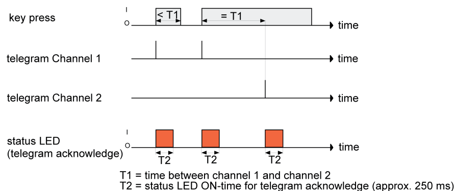
Figure 32: Example for operation concept "Channel 1 and channel 2"
