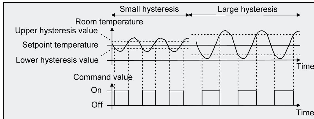
Figure 41: Effects of the hysteresis on the switching behaviour of the command value of 2-point feedback control
