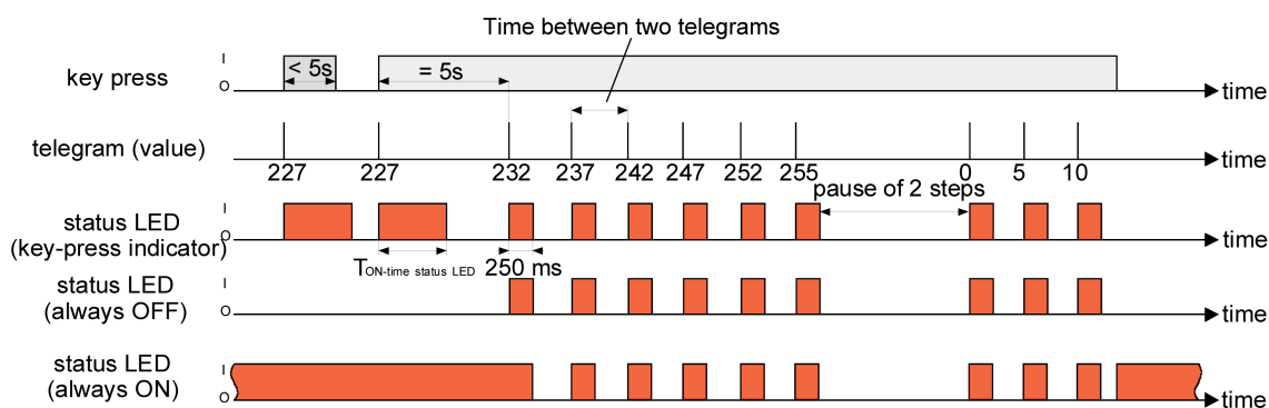
Figure 30: Example of value adjustment with value range overflow
