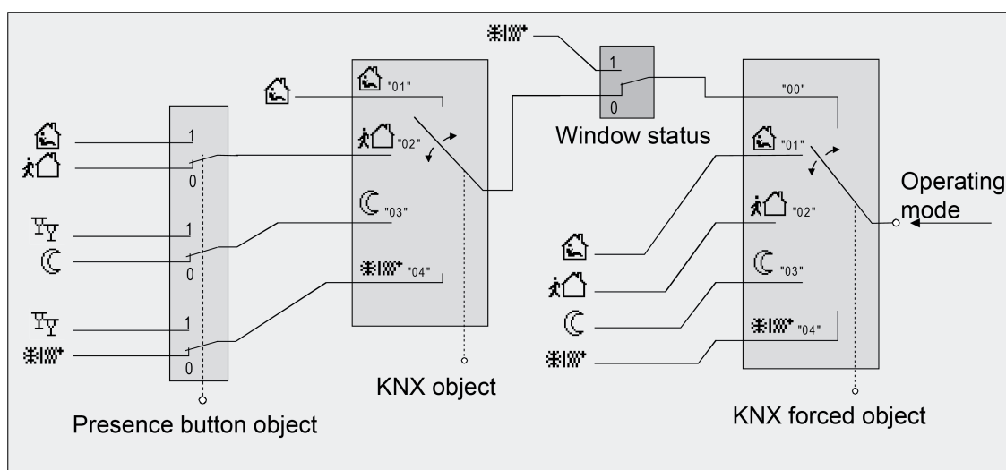
Figure 44: Operating mode change-over through KONNEX object with presence button
