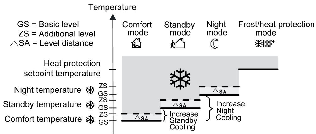
Figure 49: Setpoint temperatures in the operating mode "Basic and additional cooling"
