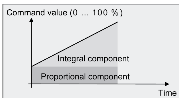
Figure 34: Continuous PI control
