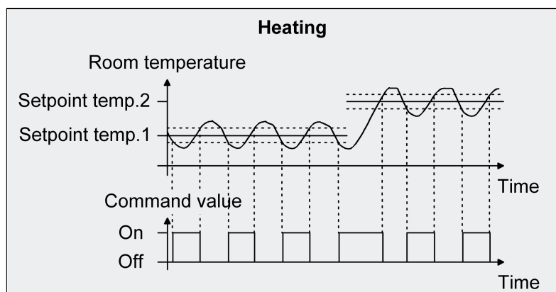
Figure 36: 2-point feedback control for the single "Heating" operating mode
