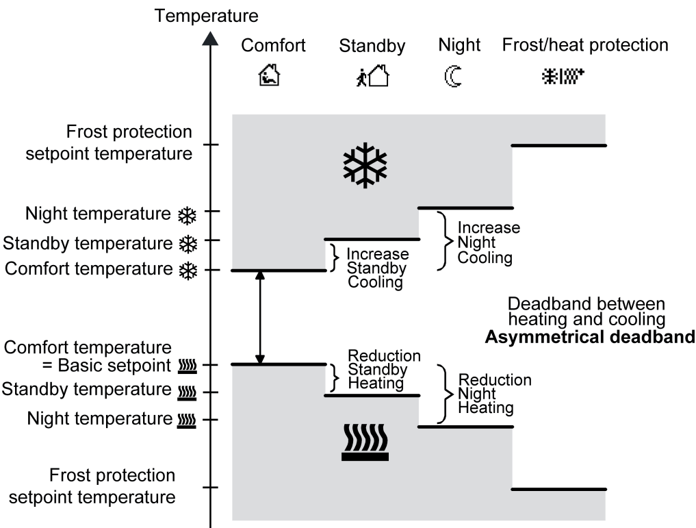
Figure 51: Setpoint temperatures in the operating mode "Heating and cooling" with asymmetrical deadband
