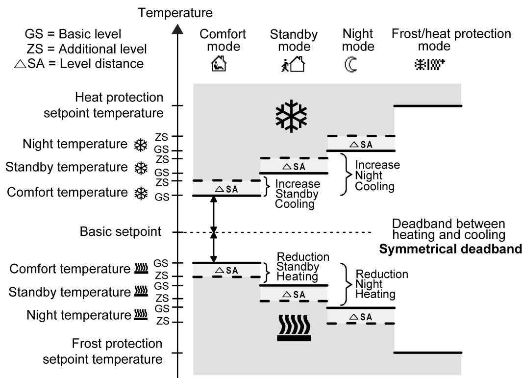
Figure 42: Setpoint temperatures in the operating mode "Basic and additional heating and cooling" with symmetrical deadband
