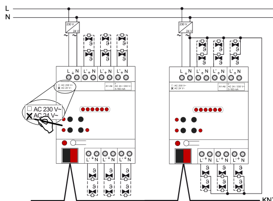
Figure 4: Raccordement de servomoteurs 24 V AC
