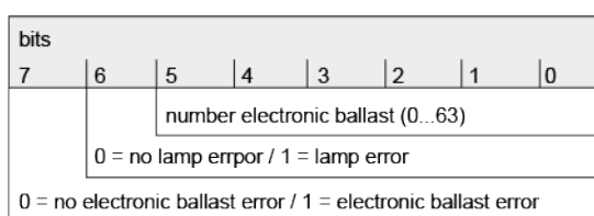
Figure 15: Telegram structure, 1-byte error status
