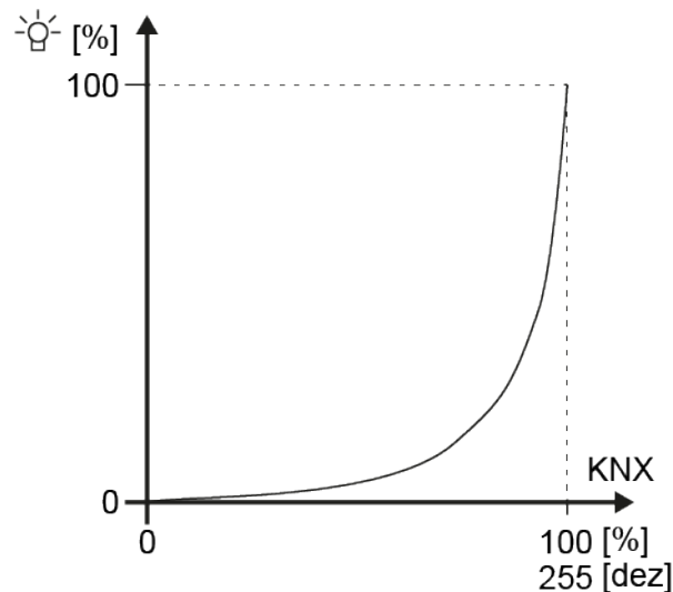
Figure 22: Logarithmic dimming characteristic curve at the output of an operating device (relative luminous flux [%] depending on the 8-bit KNX data value [0...255])
