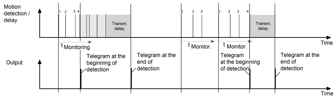
Figure 28: Motion evaluation with the detector
