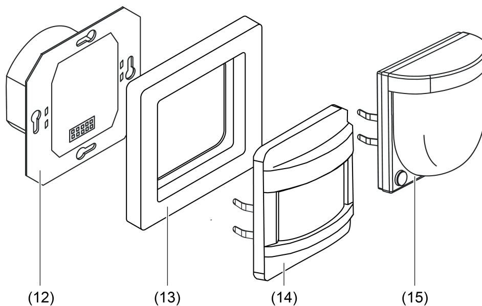
Figure 17: Mounting
