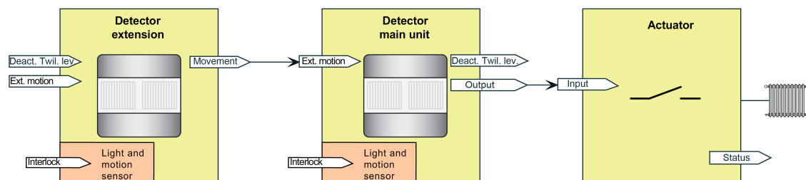
Figure 43: Application example without twilight level evaluation in the main unit and extensions
