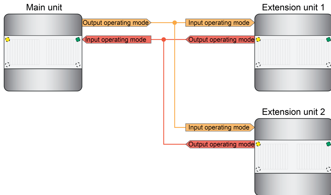
Figure 35: Example of the linking of a main unit with two extensions for operating mode switchover and display
