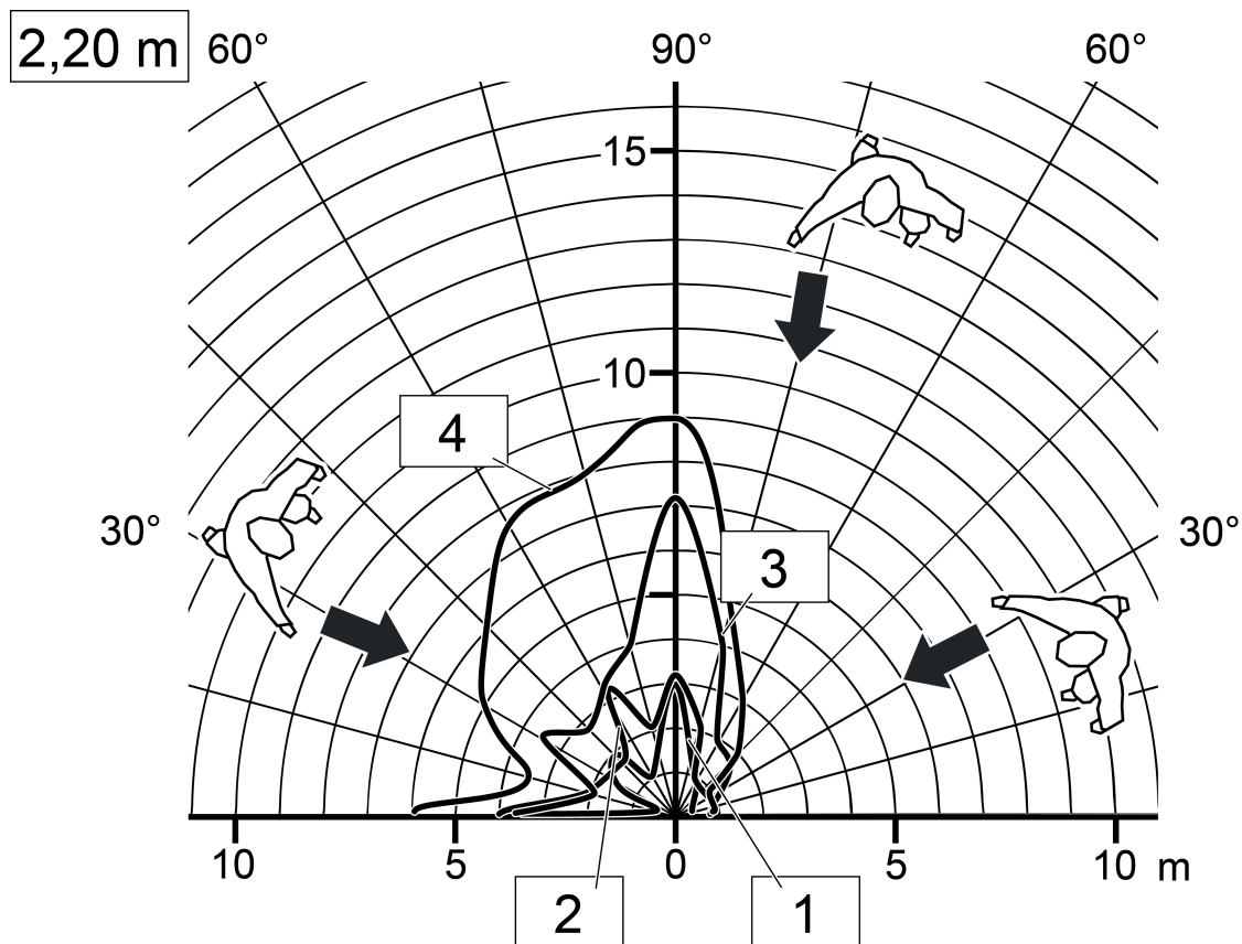
Figure 16: Range with radial direction of motion, device variant 2.20 m, mounting height 2.20 m, only one sensor active
