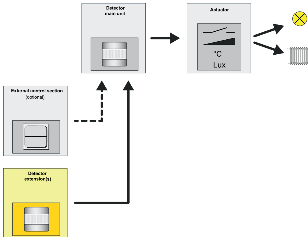
Figure 31: Application type "Extension"
