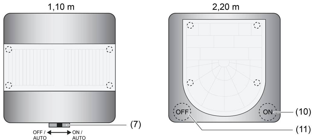
Figure 33: Arrangement of the operating elements for local operation (operating mode switchover)
