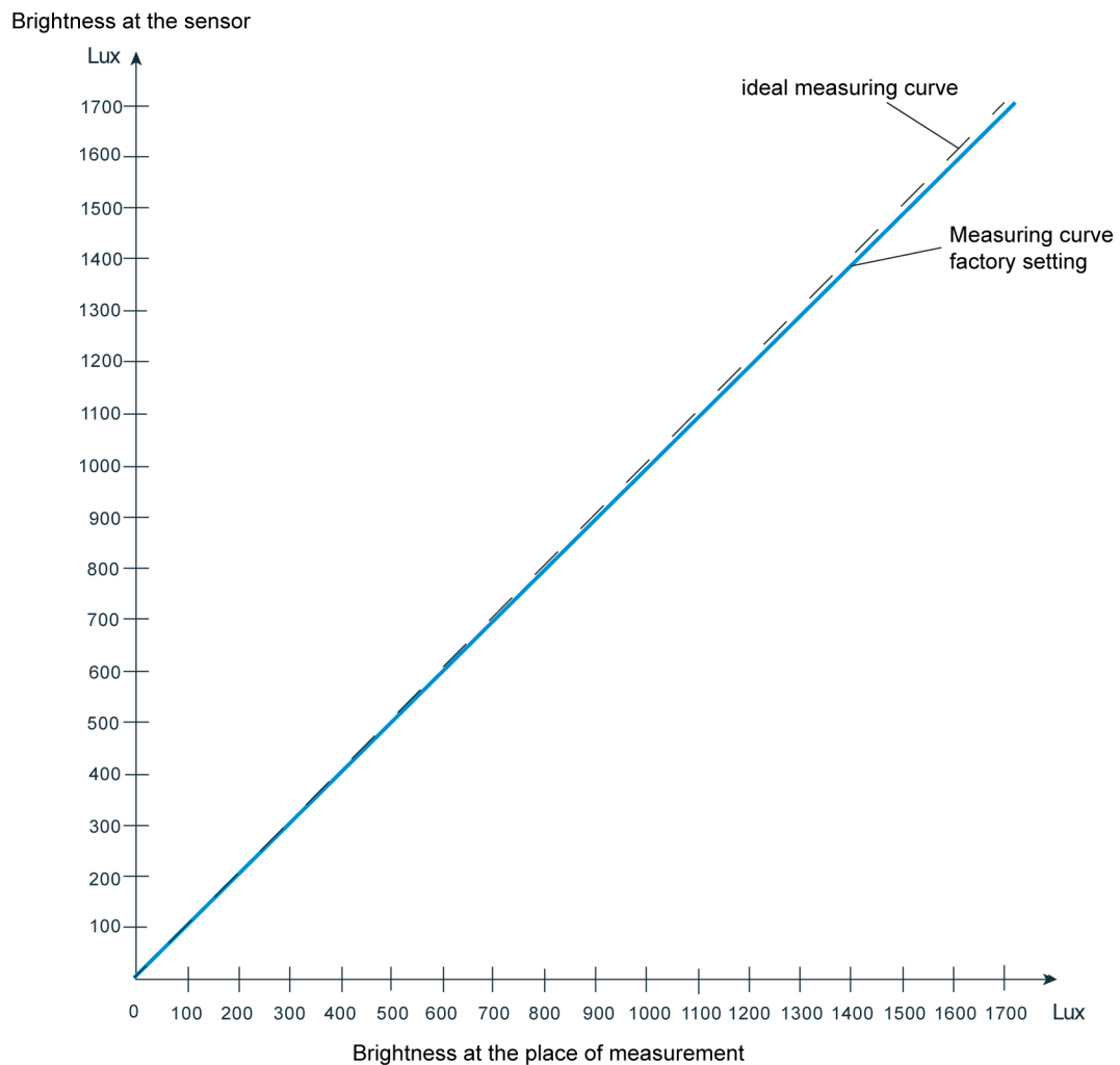
Figure 22: Measurement characteristic after factory setting (sensor measured value = ambient brightness = Ideal measurement characteristic)
