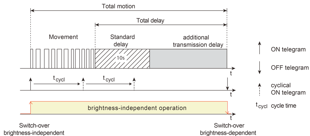
Figure 44: Total motion with motion detection, standard delay and additional transmission delay
