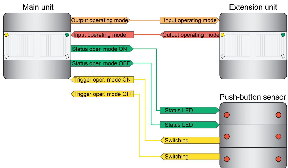
Figure 36: Example of the linking of a main unit with an extension and a pushbutton for operating mode switchover and display
