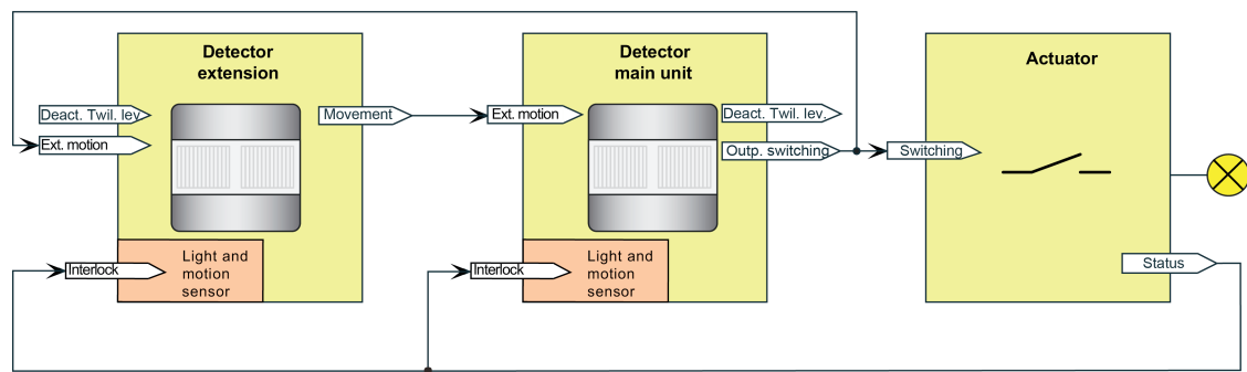
Figure 42: Application example with twilight level evaluation in the main unit and extensions for output function "Staircase function"
