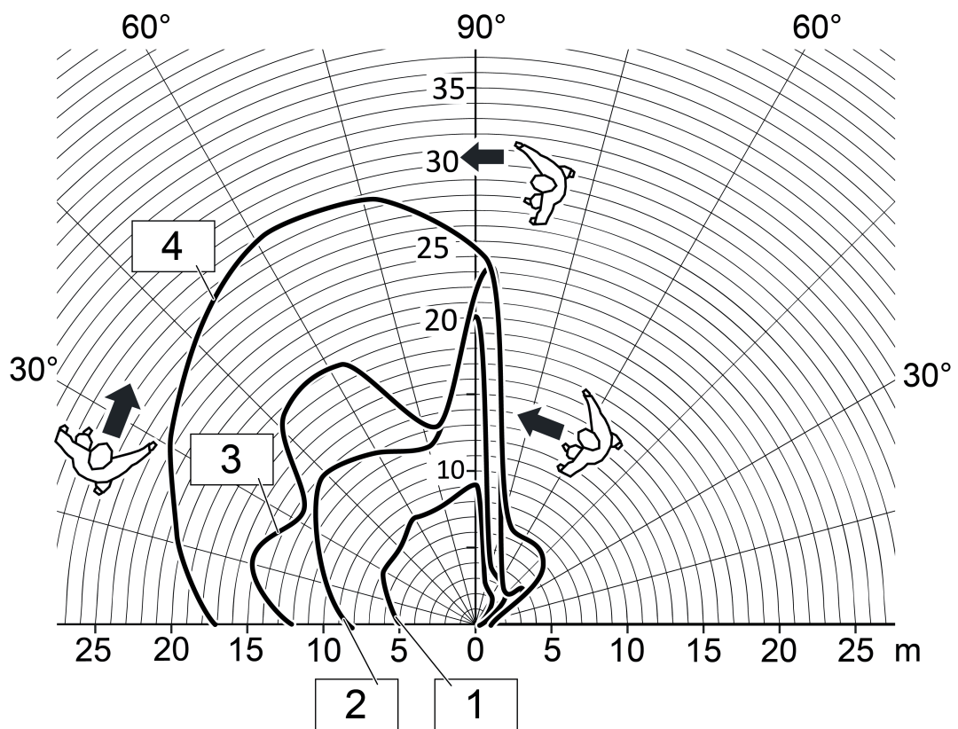
Figure 13: Range with tangential direction of motion, device variant 1.10 m, only one sensor active
