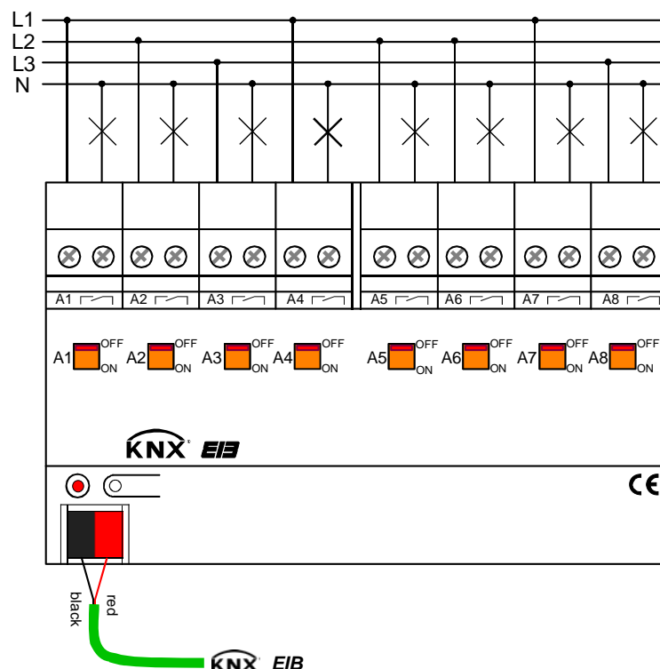
Fig. 1: Electrical connection
