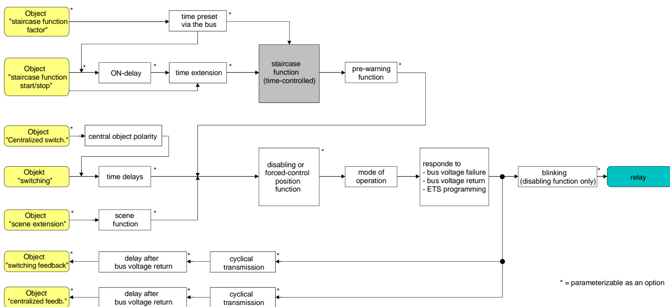
Fig. 10: Functional diagram of the staircase function
